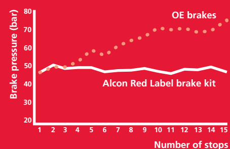
HIGH SPEED FADE TEST OVER CONSECUTIVE STOPS MAINTAINING 0.7g
